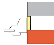
The Type FWC is introduced into the cavity after the reveal masonry is raised
