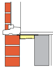
Typical application of the Type FWC used at cill level
